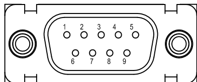
Figure 4-1 MiniScan Connector
